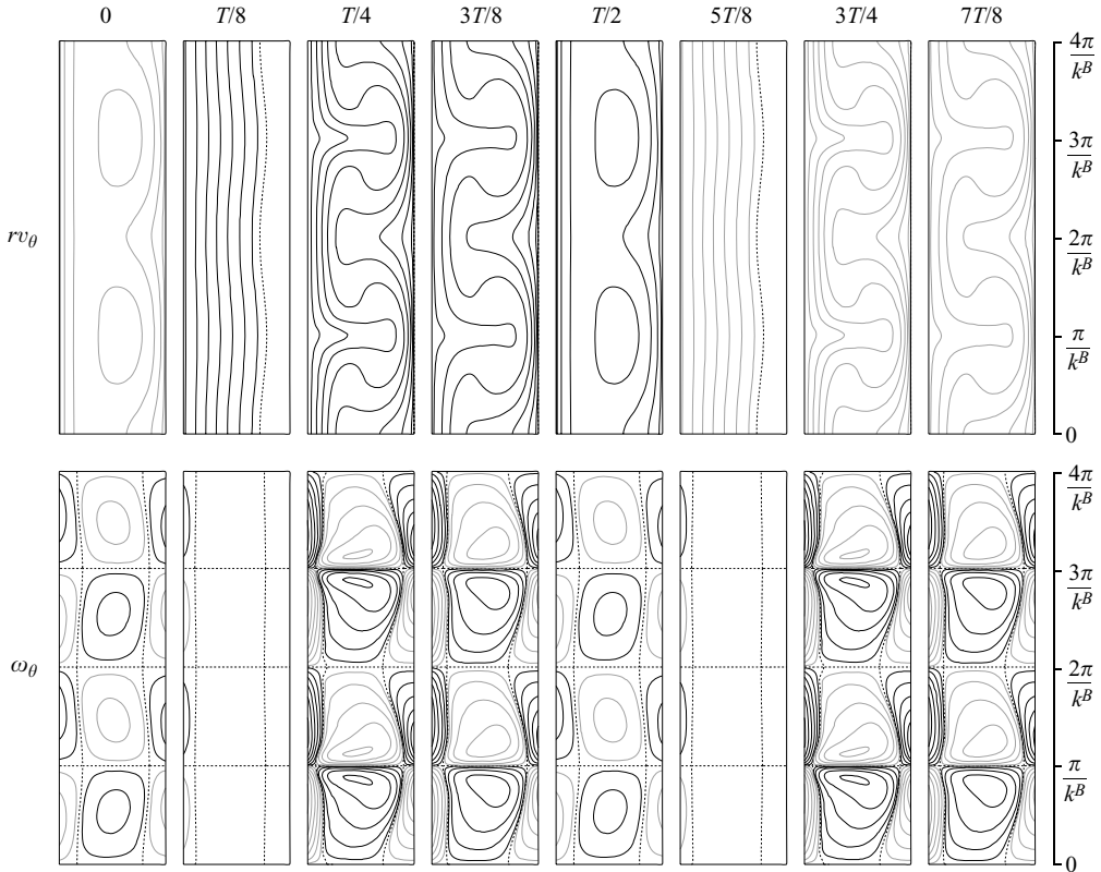
FIGURE 8. Type B (non-reversing) Taylor vortex flow at \omega = 6.1 and Re_a = 240 with wavenumber k^B = 3.4 . Quadratically spaced contours of angular momentum (top row) and azimuthal vorticity (bottom row) are shown in a meridional cross-section over a period T = 2\pi/\omega . Black (grey) contours correspond to positive (negative) values, showing r \in [1, 2] and z \in [0, 4\pi/k^B] . The snapshots have been taken after transients have vanished. In particular, a time shift of several periods t \rightarrow t - NT has been applied. (Temporal behaviour is shown in Movie 1 available with the online version of the paper).
