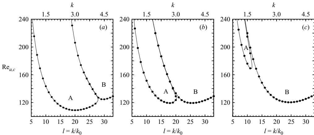
FIGURE 7. Neutral stability curves as computed with Floquet analysis for (a) \omega = 2.5 , (b) \omega = 3.936 and (c) \omega = 6 . The filled circles correspond to the discrete set of wavenumbers k considered in the nonlinear computations such that k \in [0.75, 4.95] .
