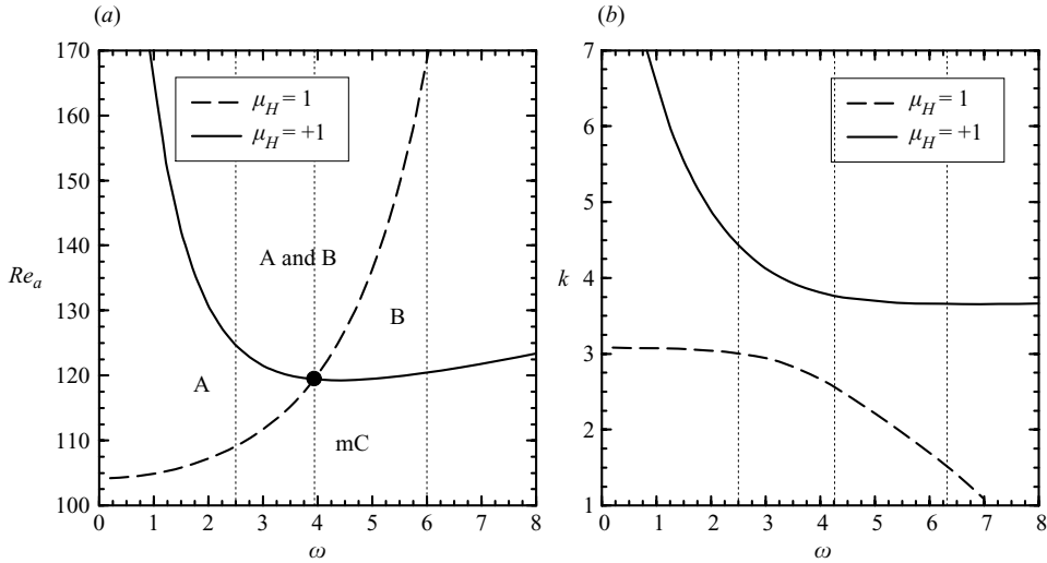
FIGURE 6. (a) Regime diagram obtained via Floquet analysis of the modulated Couette flow (2.4) using the half-period-flip map \mathcal{H} . The filled circle denotes the bicritical point (\omega, Re_{a,c}) = (3.936, 119.4) . (b) Corresponding axial wavenumber k_c(\omega) at criticality. The vertical dotted lines are the frequencies \omega at which the marginal stability curves are shown in figure 7.
