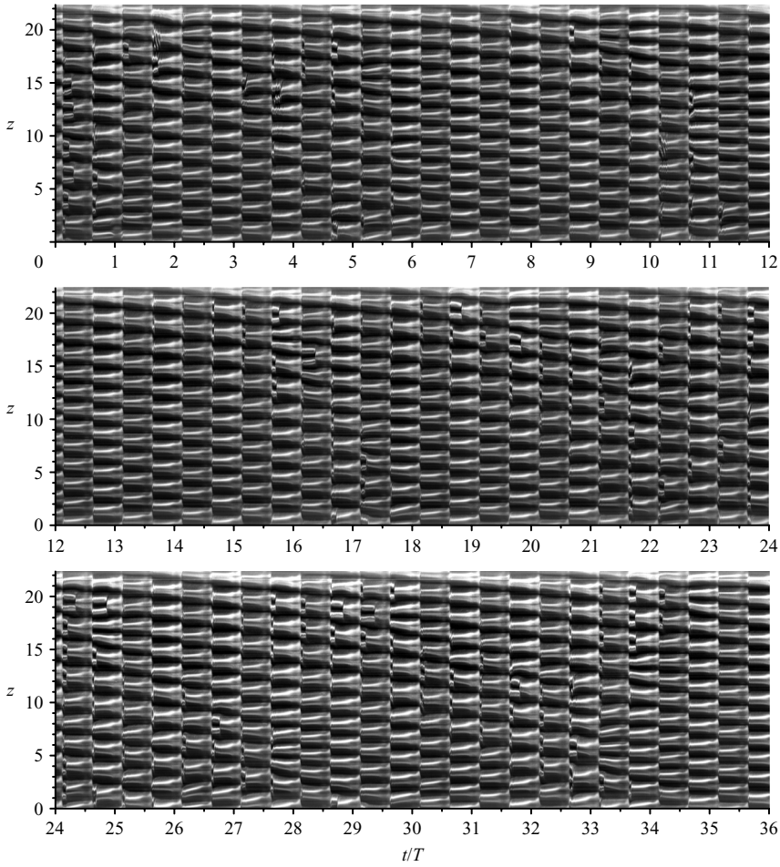
FIGURE 18. Space-time diagram showing the time evolution of a noise-sustained flow in region 4 at \omega = 2.0 and Re_a = 240 over 36 periods, corresponding to 113 viscous time units. At t/T = 0 , the frequency was changed from a stable flow at \omega = 1.0 .
