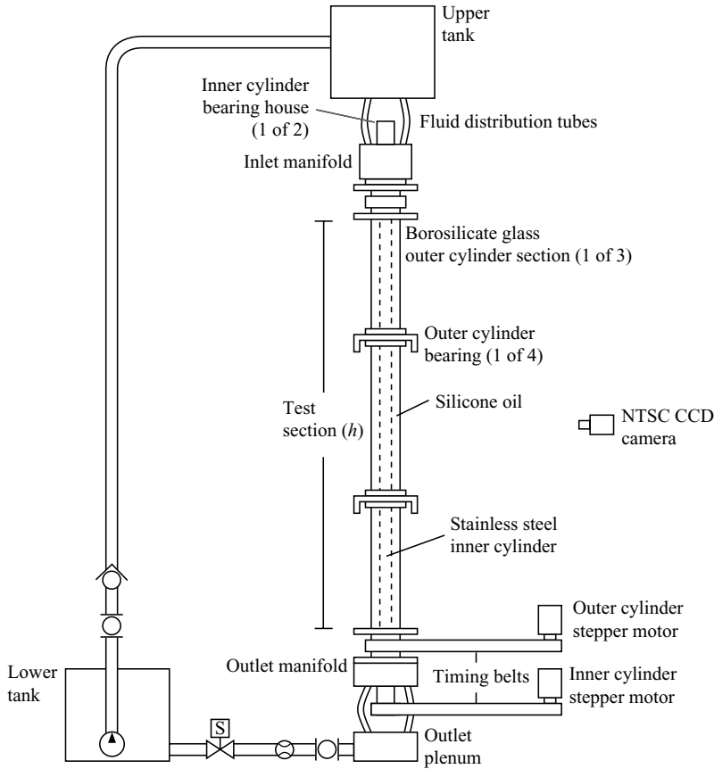
FIGURE 4. Schematic of the experimental apparatus. Overall height is approximately 4.5 m.
