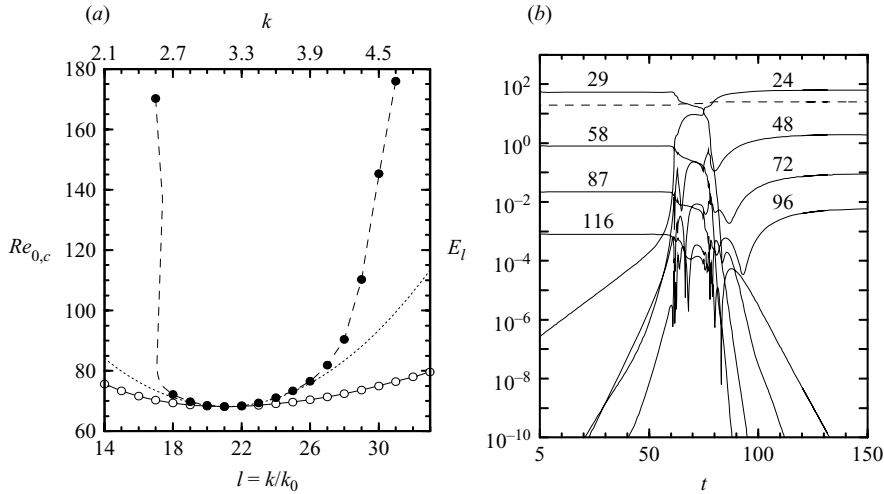
FIGURE 2. (a) Neutral (solid line) and Eckhaus (dashed line) stability curves for Couette flow with \eta = 0.5 and infinite cylinders (computations by Riecke & Paap 1986). The open and filled circles correspond to the points in these curves with axial wavenumbers in our spectral approximation (2.6), i.e. k = l k_f with k_f = 0.15 . The dotted line corresponds to the third-order Ginzburg–Landau approximation of the Eckhaus curve. (b) Solid lines show the kinetic-energy time series of the l = 24, 29 axial Fourier modes, and their three first harmonics, in the transition from the Eckhaus unstable TVF 58 to TVF 48 at Re_0 = 100 . The dashed line corresponds to the l = 0 mode.
