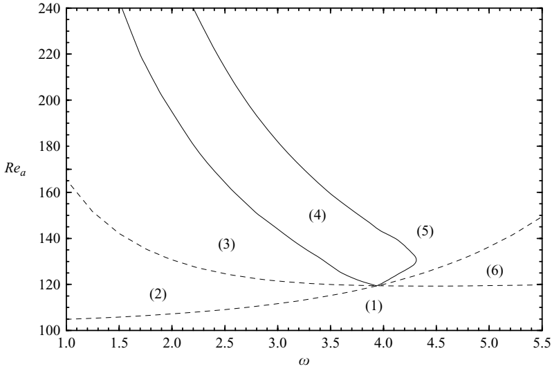
FIGURE 14. Bifurcation diagram of the competition between types A (reversing) and B (non-reversing) Taylor vortex flows. Bracketed numbers correspond to regions in parameter space with qualitatively different dynamics, described in the text. A schematic of their phase portraits is shown in figure 15.
