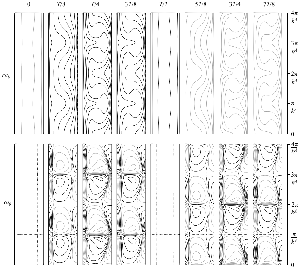
FIGURE 10. Type A (reversing) Taylor vortex flow at \omega = 1 and Re_a = 240 with wavenumber k^A = 3.0 . Quadratically spaced contours of angular momentum (top row) and azimuthal vorticity (bottom row) are shown in a meridional cross-section over a period T . Black (grey) contours correspond to positive (negative) values, showing r \in [1, 2] and z \in [0, 4\pi/k^A] . (Temporal behaviour is shown in Movie 2 available with the online version of the paper).
