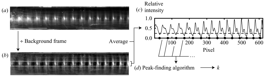
FIGURE 5. Data post-processing flow chart.
