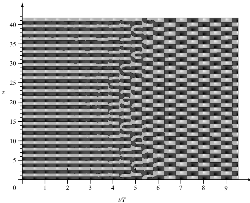
FIGURE 17. As figure 16, but the initial condition is B_{50} at \omega = 3.2 and Re_a = 140 . At t = 0 the frequency is decreased to \omega = 3.0 and the system evolves to A_{38} .
