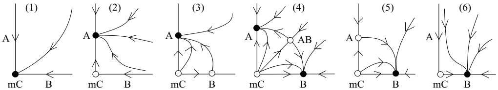
FIGURE 15. Schematic of the phase portraits of the mode competition dynamics in the six regions delimited by the bifurcation curves in figure 14. Open (closed) circles are unstable (stable) fixed points of the Poincaré map \mathcal{P} .
