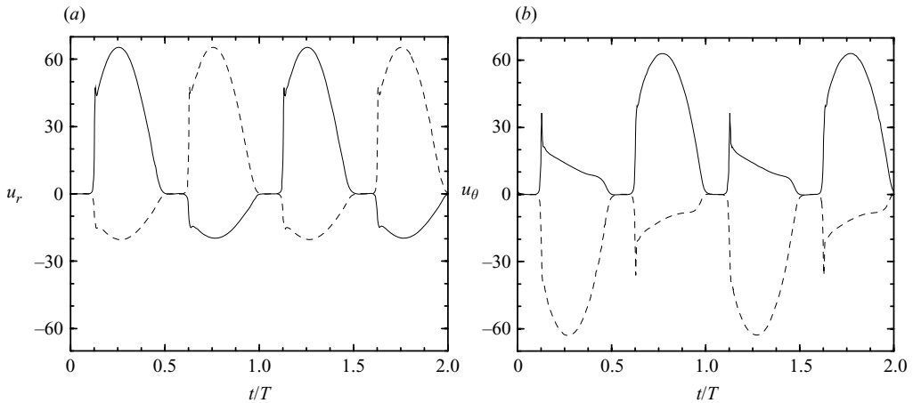
FIGURE 11. Evolution over two periods of (a) the radial velocity and (b) the azimuthal velocity components of the perturbation field (2.5) recorded at (r, \theta, z) = ((r_i + r_o)/2, 0, \pi/k^A) (solid lines) and (r, \theta, z) = ((r_i + r_o)/2, 0, 0) (dashed lines) for state A in figure 10.
