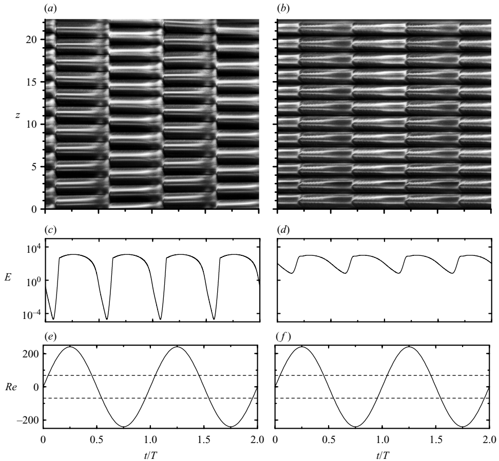
FIGURE 12. Experimental space–time diagrams of the time evolution at Re_a = 240 of (a) state A at \omega = 1 with k^A = 3.0 and (b) state B at \omega = 6.1 with k^B = 3.4 ; the corresponding computed kinetic energies of the perturbation field \mathbf{u} are shown in (c) and (d), and the corresponding instantaneous Reynolds numbers Re(t) = Re_a \sin \omega t (solid curve) are given in (e) and (f) which also include Re_{0,c} = \pm 68.19 (dashed lines).
