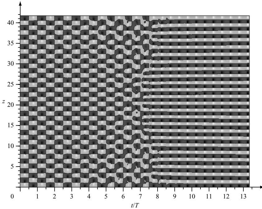
FIGURE 16. Space-time diagram showing an azimuthal vorticity colour-map at (r, \theta) = (r_o, 0) over time and the whole computational domain in the axial direction z \in [0, \Lambda] . Black (grey) corresponds to positive (negative) values. The initial condition is A_{36} at \omega = 4 and Re_a = 140 . At t = 0 the frequency is increased to \omega = 4.2 and the system starts evolving to B_{48} .
