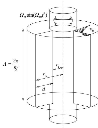
FIGURE 1. Schematic of modulated Taylor–Couette flow.
