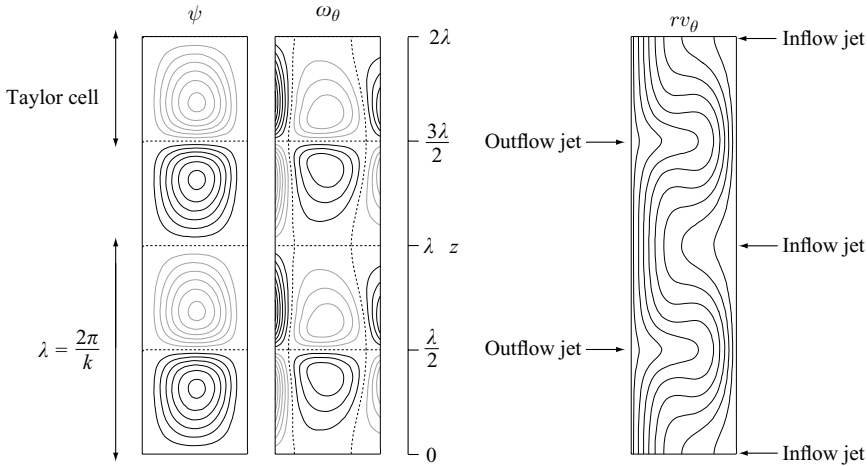
FIGURE 3. Taylor vortex flow (TVF 42 ) at Re_0 = 100 with axial wavenumber k = 3.15 . Contours of the streamfunction \psi and azimuthal vorticity \omega_\theta are shown in a meridional cross-section. Vortex lines ( rv_\theta contours) show the outflow and inflow jets separating the Taylor cells. Black (grey) contours correspond to positive (negative) values, showing r \in [1, 2] and z \in [0, 2\lambda] .
