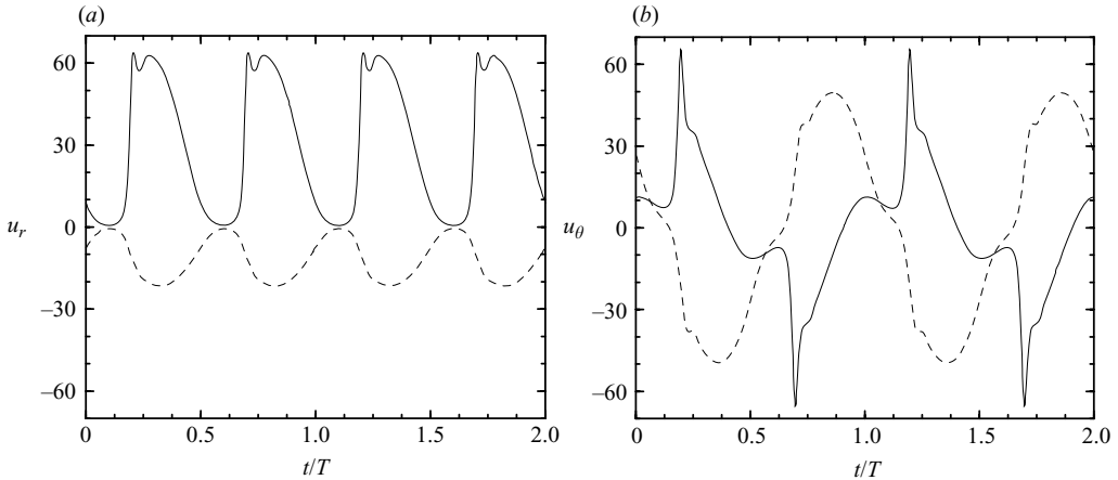
FIGURE 9. Evolution over two periods of (a) the radial velocity and (b) the azimuthal velocity components of the perturbation field (2.5) recorded at (r, \theta, z) = ((r_i + r_o)/2, 0, \pi/k^B) (solid lines) and (r, \theta, z) = ((r_i + r_o)/2, 0, 0) (dashed lines) for state B in figure 8. Note that the time axes have been normalized by the period T .
